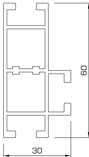
193 - Upright or rail
