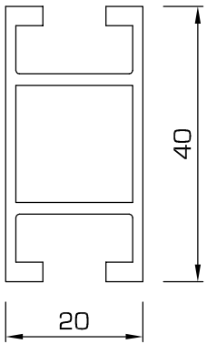
92 - Upright or rail
