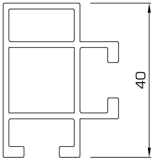
93S - Upright or rail
