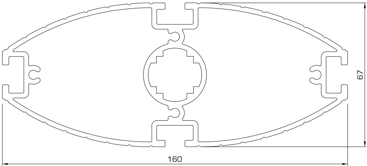
164 - Upright, large elliptical profile with ribbed finish
