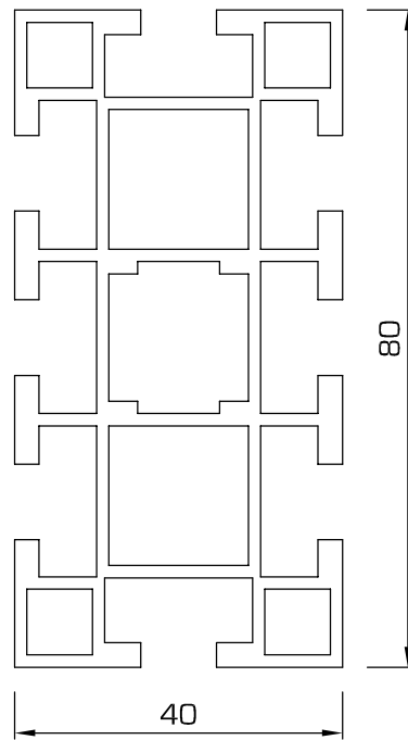
294 - Upright or rail, for larger structural designs
