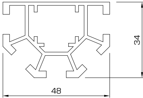
85 - Upright, 180°
