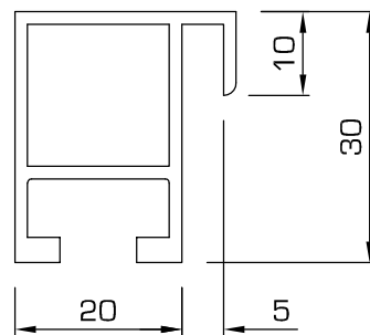
91D - Sign profile for 4mm panels
