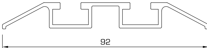
102 - Threshold rail with twin channel
