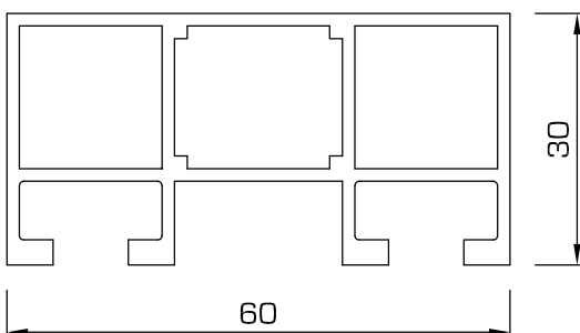
92LL - Upright or rail, double 90° corner
