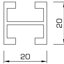
02 - Twin channel
