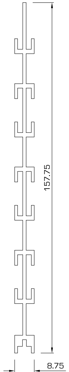
SLOT - Slotwall adaptor - fits together vertically to produce slatwall to any required height
