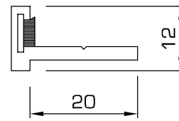
105 - Doorstop with wool pile
