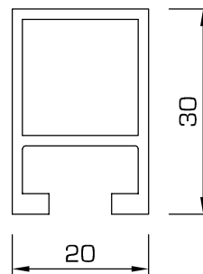
91 - Upright or rail
