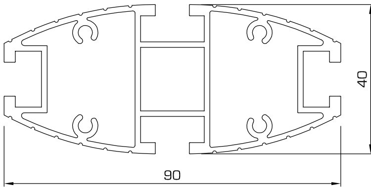
190 - Upright, small elliptical profile with ribbed finish
