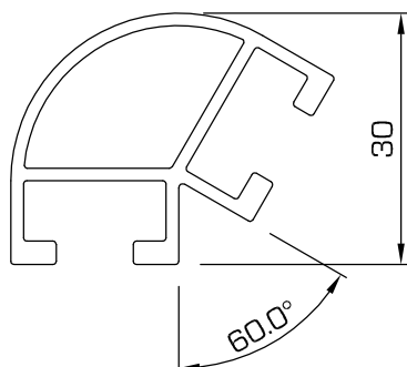
62 - Upright, 60° corner
