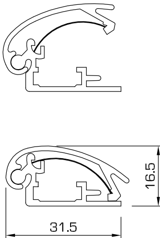
D10R - Clip frame with curved front
