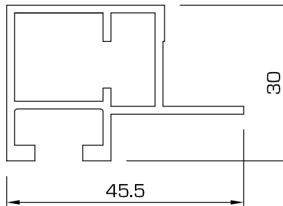
92LF - Rail, 90° corner with flange
