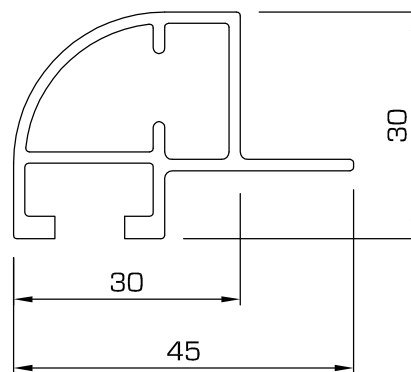
92LRF - Rail, 90° corner with flange
