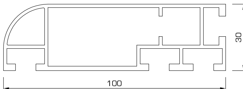
92LRC - Extra wide profile (for wall mounted showcases)
