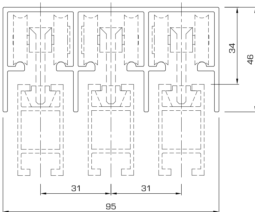
73 - Triple channel sliding door track.
