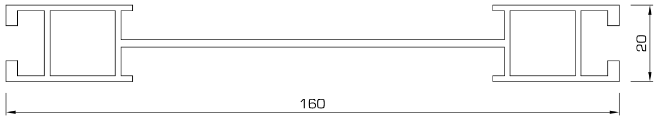
160 - 100mm deep fascia rail
