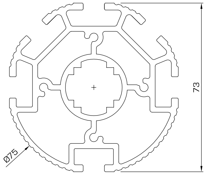
76 - Upright, six-way circular profile with ribbed finish
