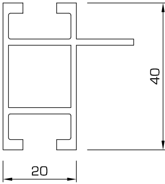
92F - Rail, with flange
