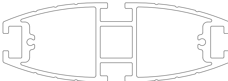
124 - Upright, medium elliptical profile with ribbed finish
