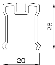
S01 - Aluminium trim for post profile S40
