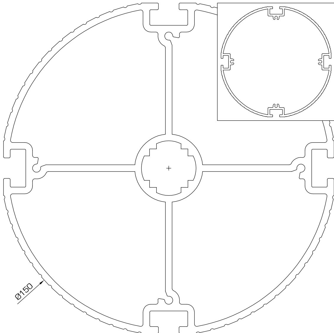
180 - Upright, large circular profile with ribbed finish with central boss
