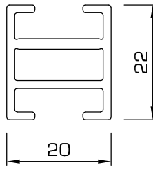
92A - Upright or rail, use 600AC connector
