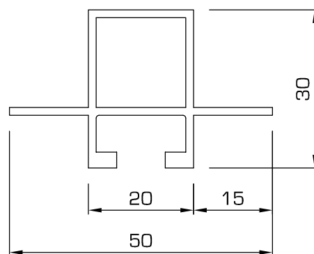
91FF - Rail, with twin flange
