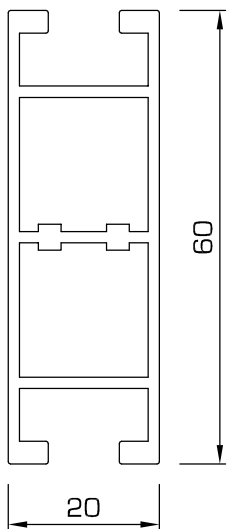
192 - Upright or rail
