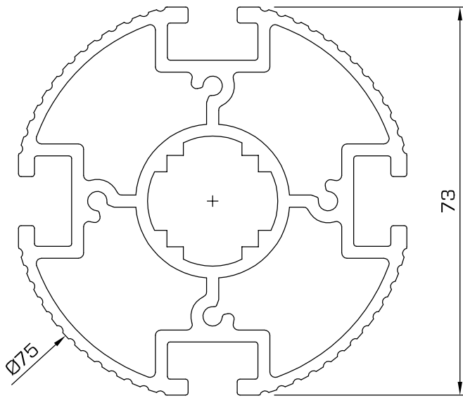
74 - Upright, four-way circular profile with ribbed finish
