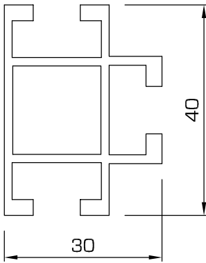
93 - Upright or rail
