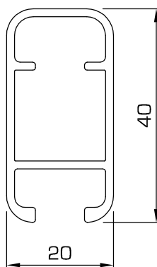
60 - Upright or rail, 90° corner
