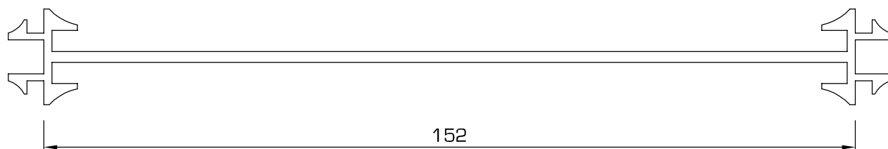
150D - Decorative infill that slides in FOGA channels, can be used vertically or horizontally
