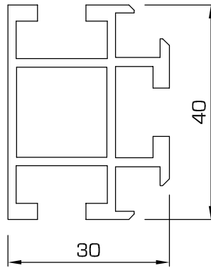
93R - Upright, with shelf support
