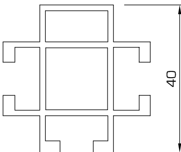
94S - Upright or rail
