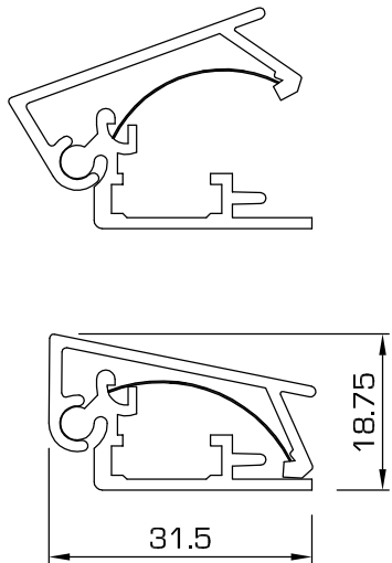
D10 - Clip frame with flat front
