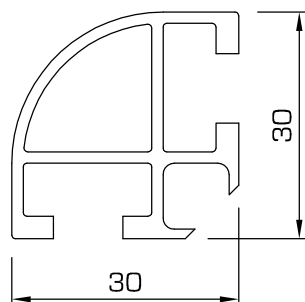
92LR - Upright or rail, 90° corner with shelf support
