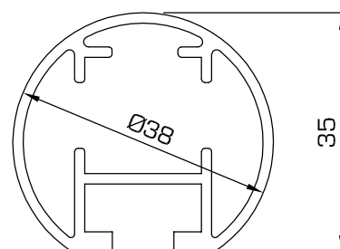
151 - Upright or rail, round
