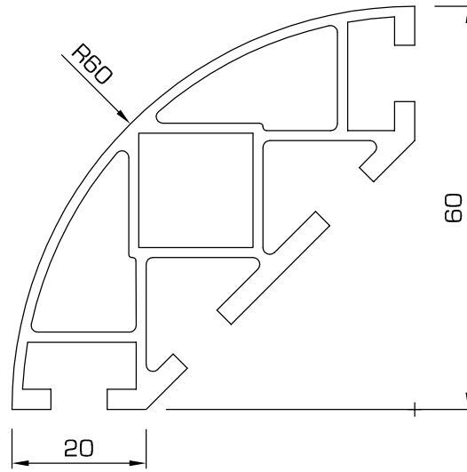
292S - Upright or rail, large 90° corner
