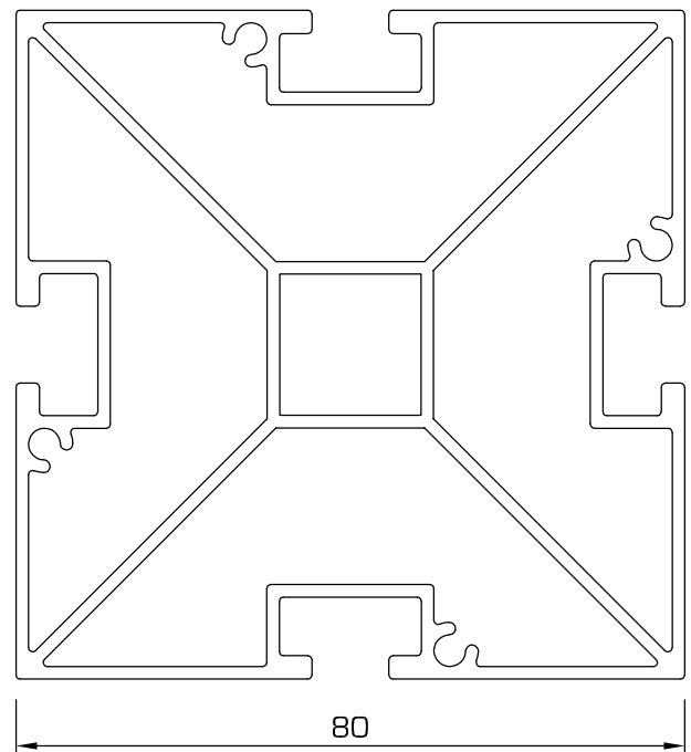
80S - Upright or rail, square
