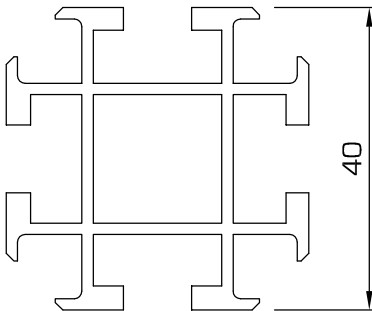
94R - Upright, with shelf support
