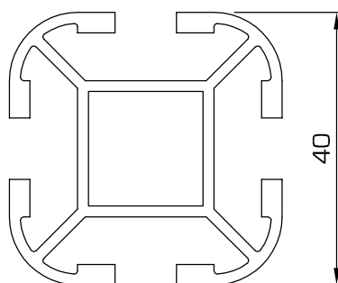
154 - Upright or rail, square, radius corners
