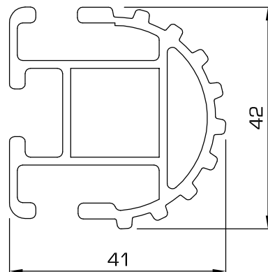
33 - Gear edged, produces hinge
