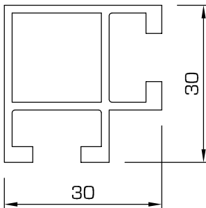
92L - Upright or rail, 90° corner
