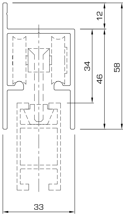
70 - Single channel sliding door track
