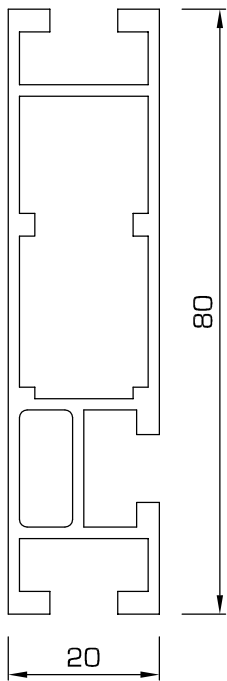
293 - Upright or rail
