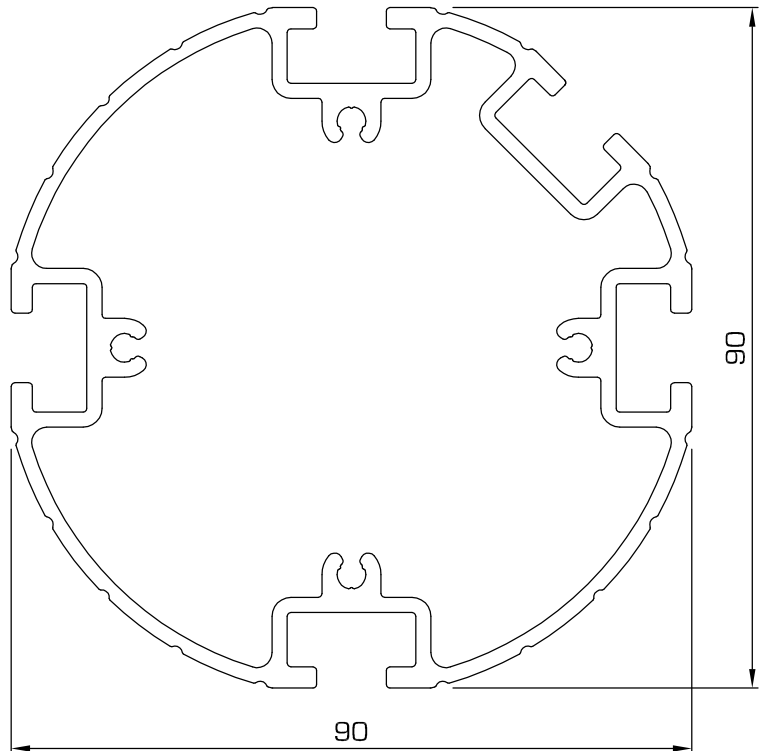
95 - Upright, medium circular profile with ribbed finish
