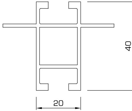
92FF - Rail, with twin flange
