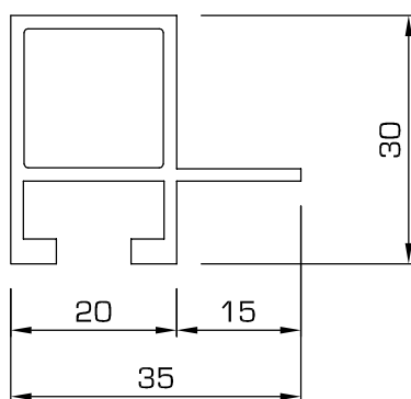
91F - Rail, with flange
