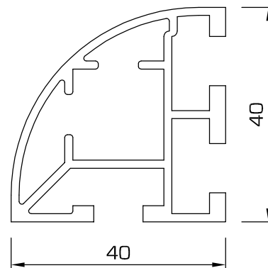
194R - Upright or rail, 90° corner
