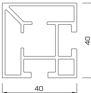
51 - Upright or rail, one-way, radius corners
