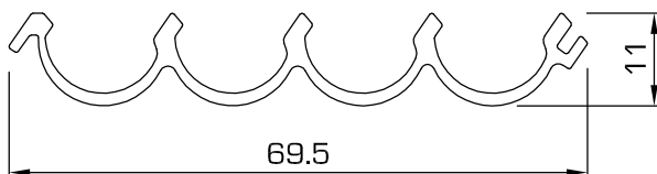
DVD Holder - For browsing DVDs in standard cases
