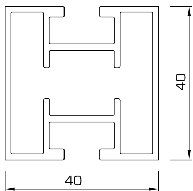
43TX - Forms tensioned fabric walls, use with 613 connector and 350TX silicone strip
