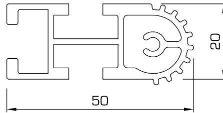
21-3 - Gear edged, produces hinge
