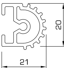
21A - Gear edged, produces hinge. Use with 600AC coupling and profiles 91A and 92A
