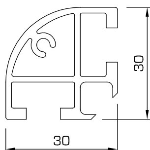
92LRS - Upright or rail, 90° corner with shelf support and screw port
