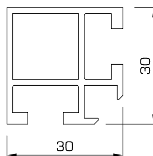
92R - Upright or rail, 90° corner with shelf support
