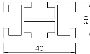
04 - Four-way channel
