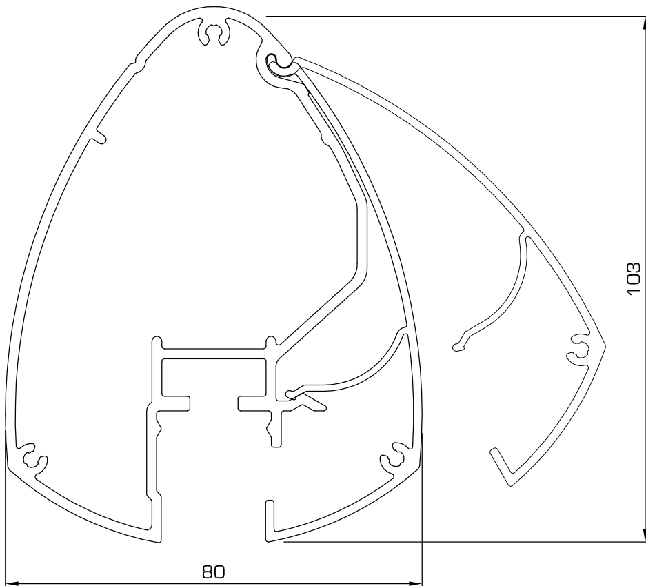
S40 - Post profile, specially for signs
