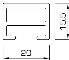
91A - Upright or rail, use 600AC connector
